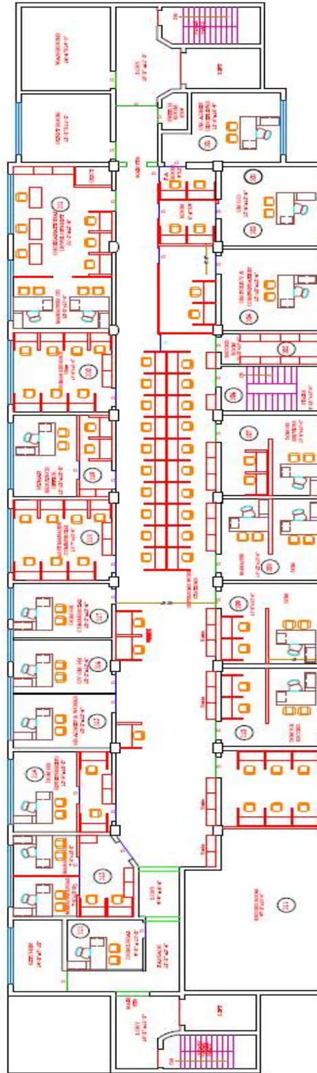
2ND FLOOR PLAN (PROPOSED) 85 Persons Sitting Capacity on Floor
